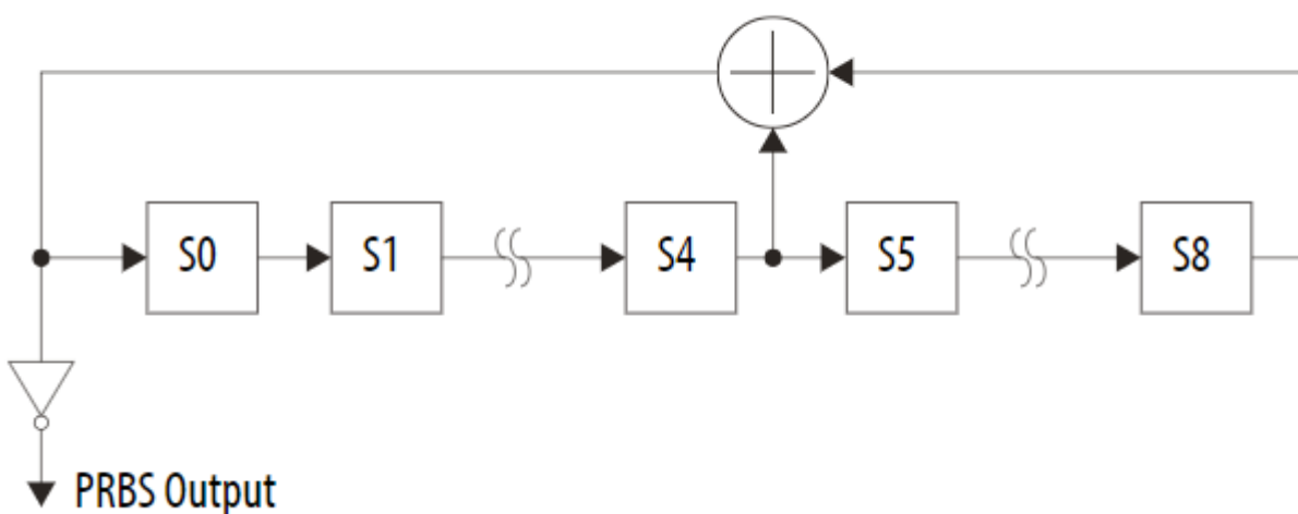
Figure 227. PRBS Generator for Serial Implementation of PRBS9 Pattern
