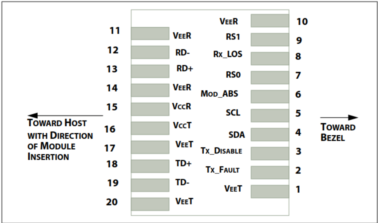
Figure 1 Host PCB SFP+ pad assignment top view
